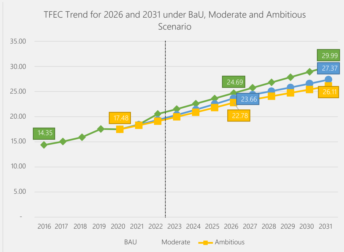
Figure 18 TFEC Trend for 2026 and 2031
