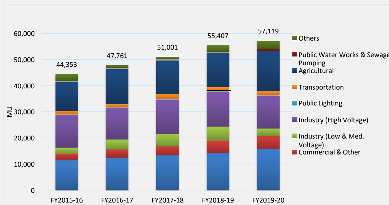
Figure 5 Electricity consumption of Andhra Pradesh over a period of FY 2015 to FY 2020 9
